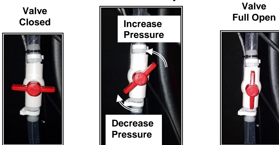
Diagram 8B Flow Control Valve Adjustment
